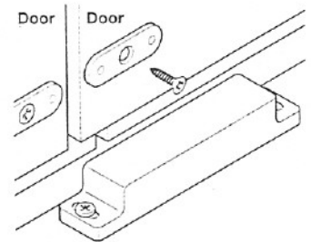
Strike
